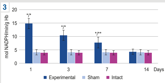
Fig. 3. Glutathione reductase activity in rat erythrocytes. *: p < 0.01 between the Experimental and Sham / Intact groups; **: p < 0.05 between the Experimental and Intact groups.
