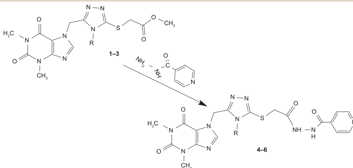
Fig. 1. The scheme of synthesis of N -(2-(5-((theophylline-7'-yl)methyl)-4- R -4 H -1,2,4-triazole-3-ylthio)acetyl)isonicotinohydrazides.
